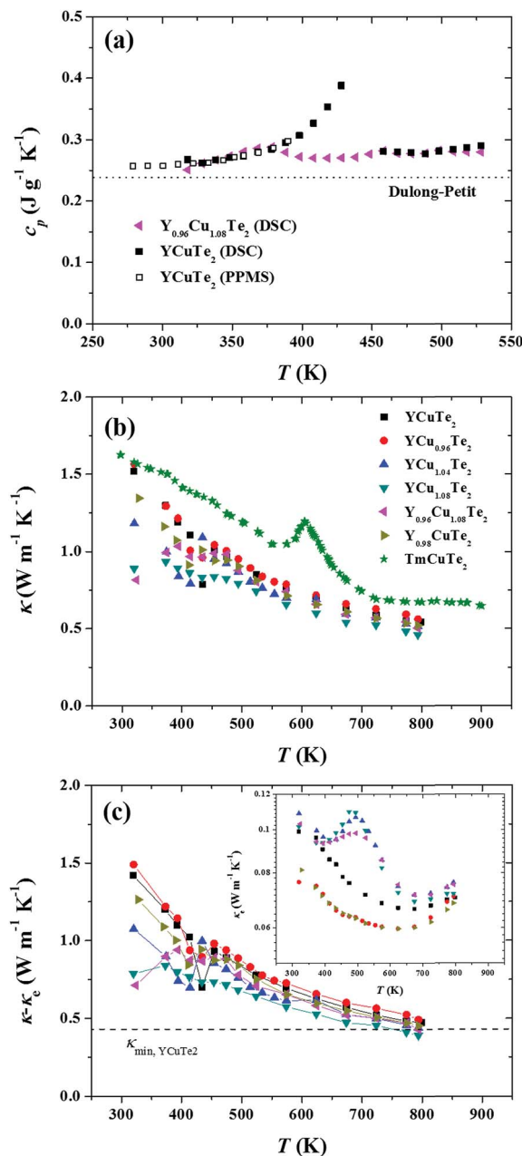
Fig. 12 (a) Heat capacity of YCuTe 2 (parent compound) and Y 0.96 Cu 1.08 Te 2 . A phase transition was observed for the parent compound at \sim 440 K, whereas Y 0.96 Cu 1.08 Te 2 shows only a subtle anomaly at \sim 370 K, consistent with the DSC results. (b) The thermal conductivity of YCuTe 2 compounds decreases with increasing temperature. The room-temperature thermal conductivity decreases with increasing Cu content and decreasing Y content. All samples display lower \kappa than that of TmCuTe 2 . (c) The phononic contribution of the thermal conductivity, determined from the experimental thermal conductivity with the calculated electronic contribution (see text) subtracted, approaches the predicted minimum thermal conductivity. Inset: the electronic contribution of the thermal conductivity indicates a peak for Cu-excess (YCu x Te 2 , x > 1 ) samples above the phase transition.
